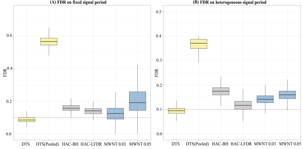
Figure 1. For independent streams without temporal correlation, (N, p) = (4800, 800) , \sigma^2(t) = 1 . (A) is the boxplot of the empirical FDR in the fixed signal period; (B) is the boxplot of the empirical FDR in the heterogeneous signal period.
