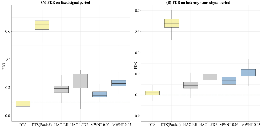
Figure 2. For dependent streams \rho_{\text{Block}} = 0.5 with temporal correlation \rho_{\text{Tempo}} = 0.5 , (N, p) = (2400, 800) , \sigma^2(t) = 8 . (A) is the boxplot of the empirical FDR in the fixed signal period; (B) is the boxplot of the empirical FDR in the heterogeneous signal period.
