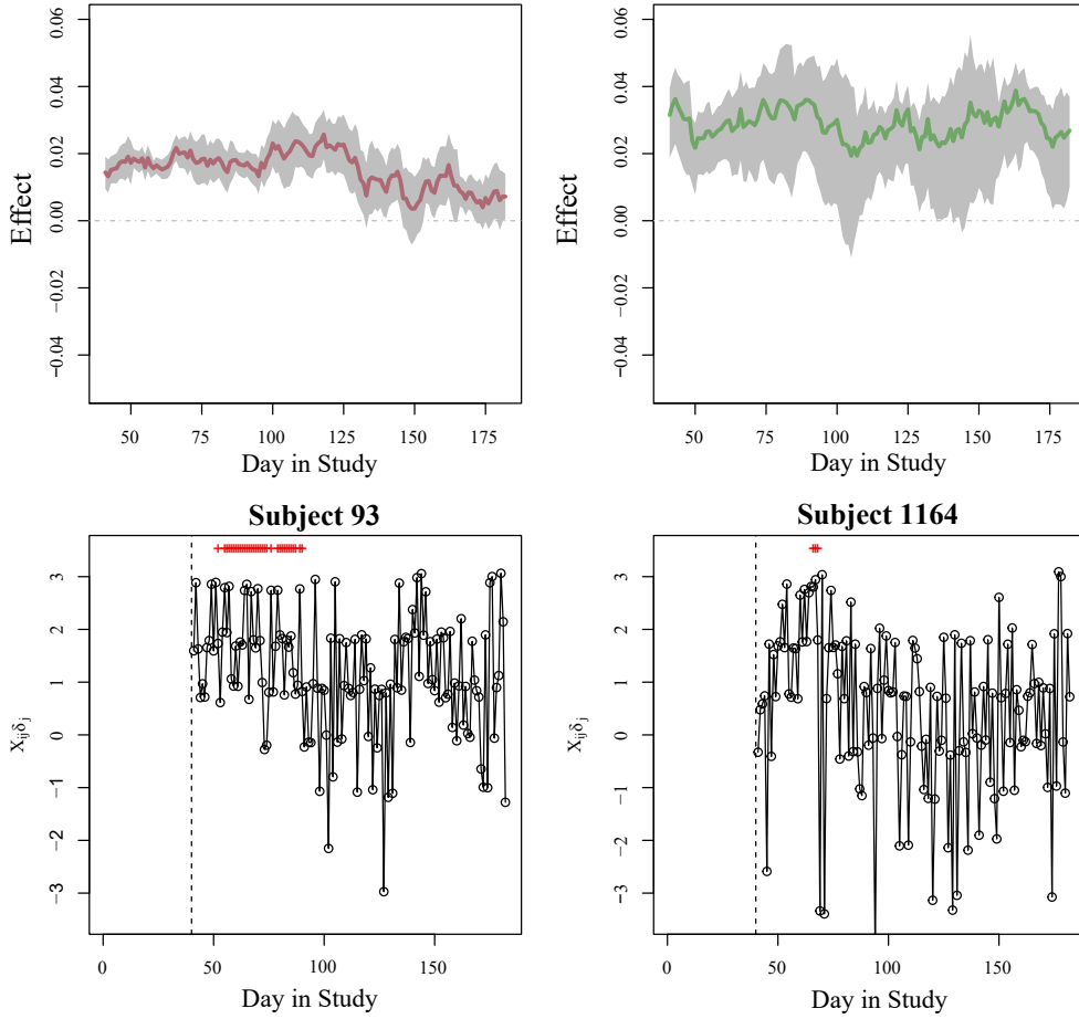
Figure 5. Upper panels: the estimated main time-varying effects for step counts (left; cubic root scale) and sleep hours (right; square root scale). Lower panels: the estimated X_{ij}^T \delta_j(t_i) for two random subjects. The red horizontal pluses indicate the days with detected deviation from the population model; both are online estimates/decisions.
