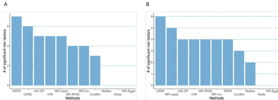
Figure 4. Number of significant causal pairs identified by different methods under Bonferroni-correction threshold < 0.05/45 \approx 10^{-3} using (A) 45 exposures used in negative control analysis and (B) 24 exposures that are reported by CDC and existing literature.
