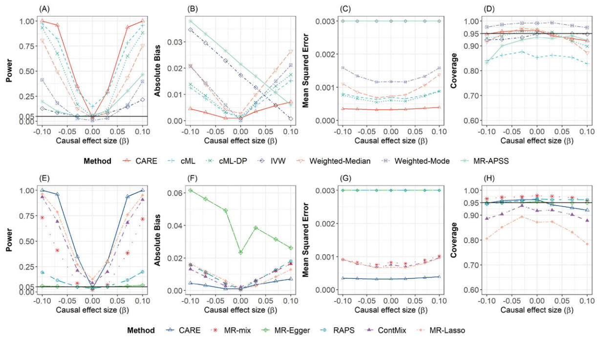
Figure 2. Power, absolute bias, mean squared error, and coverage of the CARE estimator and several robust MR methods under the main setting with 50% invalid IVs. Power is the empirical power estimated by the proportion of p -values less than the significance threshold of 0.05. Coverage is the empirical coverage probability of the 95% confidence interval.
